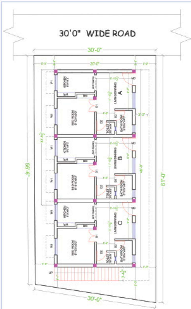
SITE CUM GROUND FLOOR PLAN - PLOT No. 36
