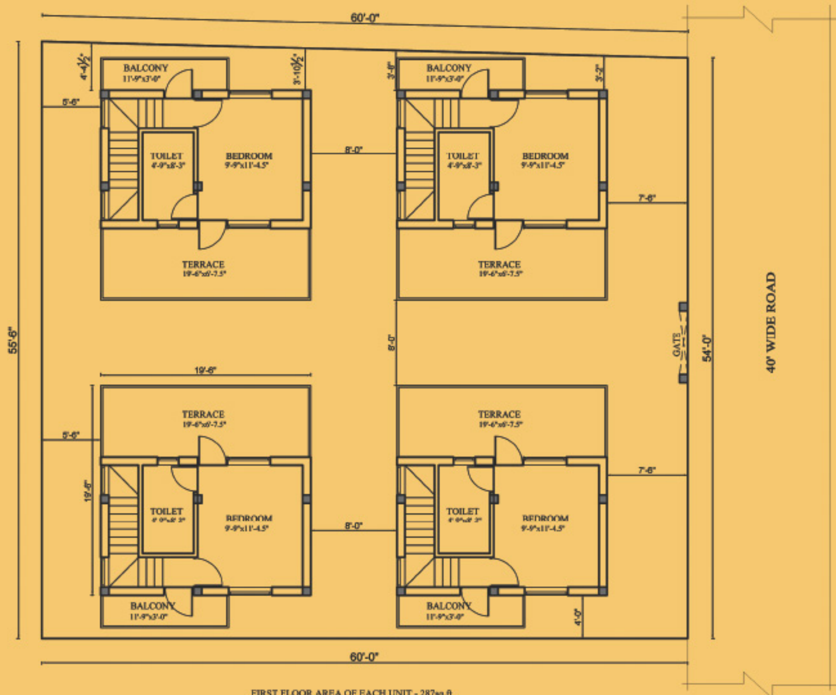
FIRST FLOOR AREA OF EACH UNIT - 287sq. ft.
